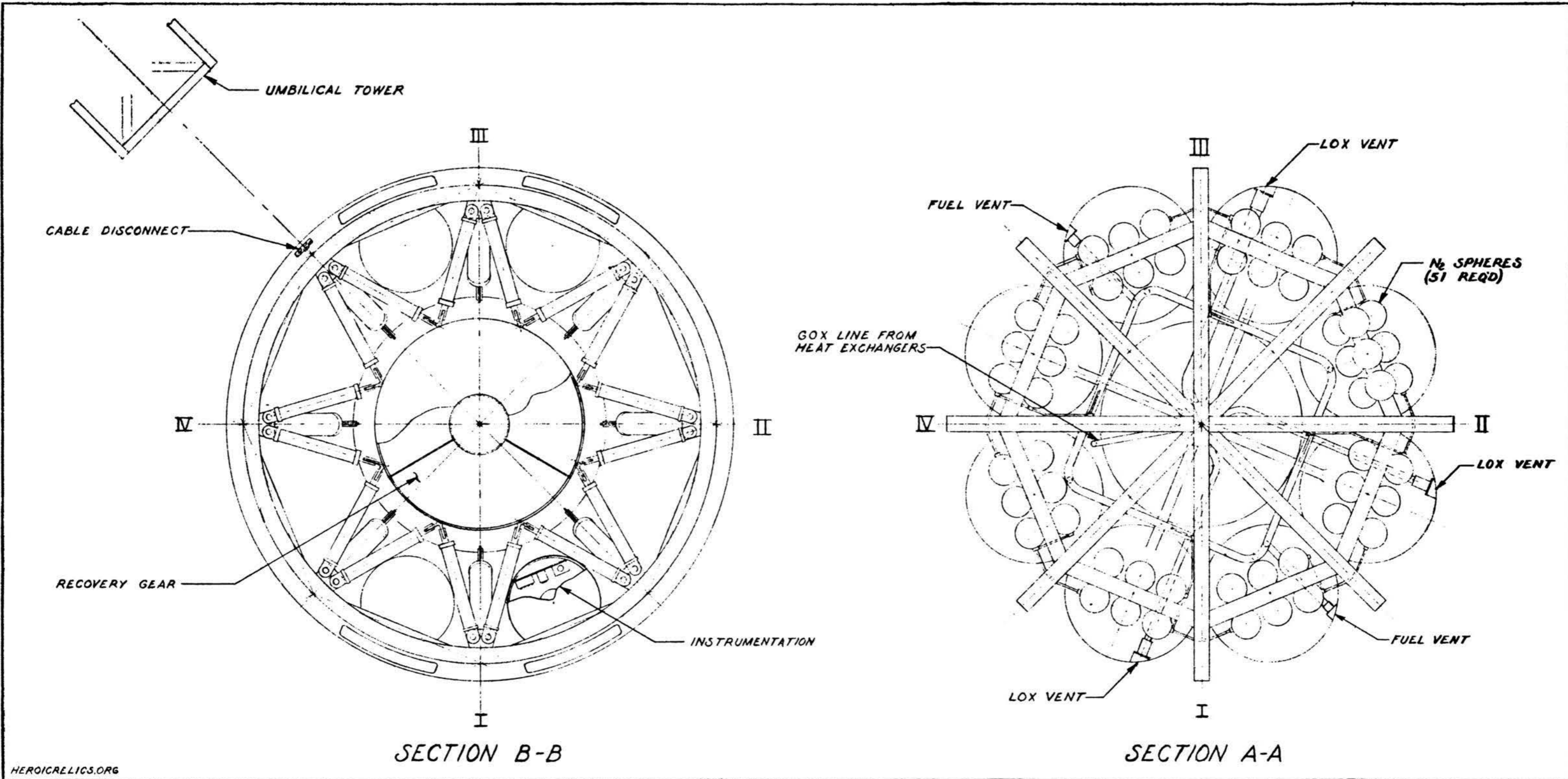
Figure 2-2. Booster Configuration Data (Part I)
