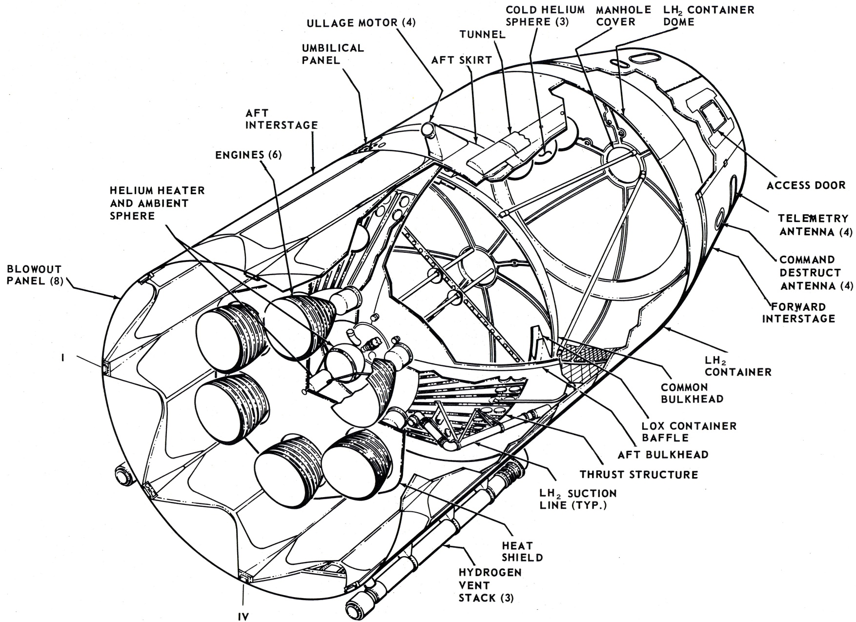
S-IV STAGE
