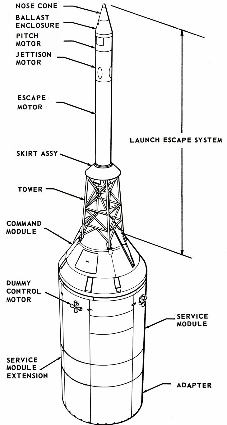
APOLLO SPACECRAFT
