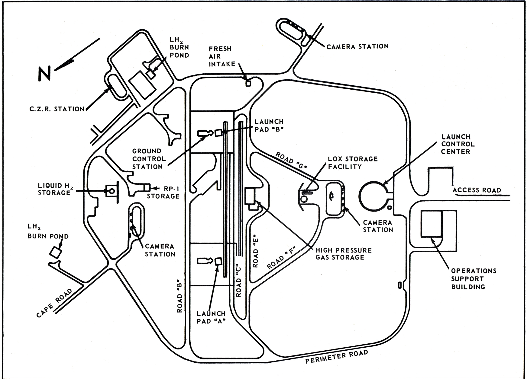
LAUNCH COMPLEX 37
