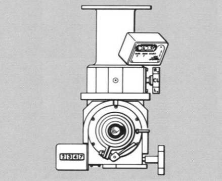
ALIGNMENT OPTICAL TELESCOPE (AOT)
