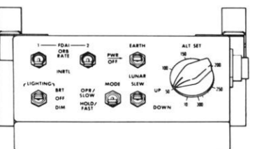
ORBITAL RATE DISPLAY — EARTH AND LUNAR (ORDEAL)
