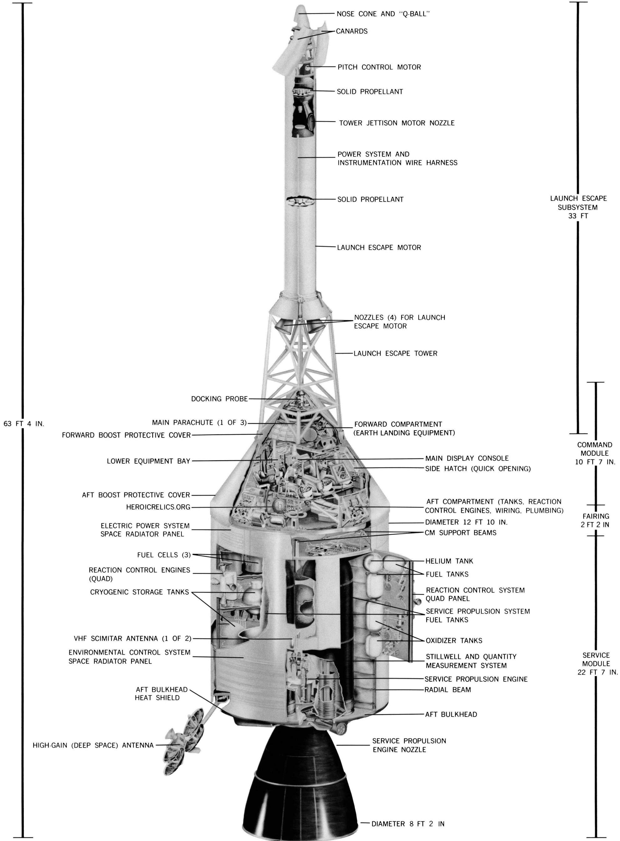
Apollo command and service modules
